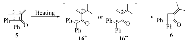
Scheme 9. Two possible intermediates ( 16 +- and 16 •• ) in the thermal rearrangement of 5
